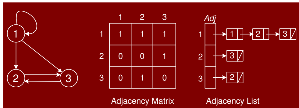
Figure 8.6: Graph Representations
